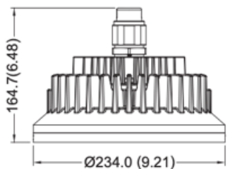
Dimension in Millimeters (inches)
